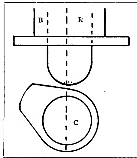
Fig. 2—Lower part of pushrod and cam. Dotted line shows wear on end of rod
